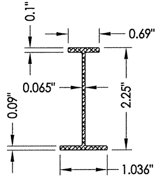
11 MULLION REINFORCEMENT
