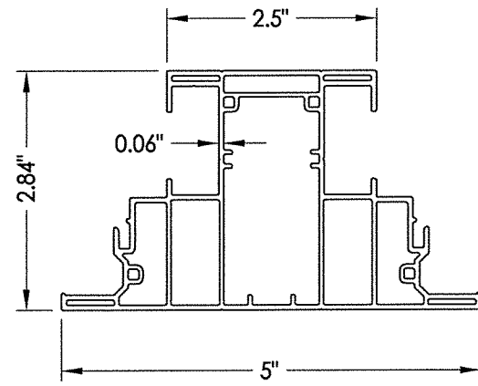
10 INTEGRAL MULLION
