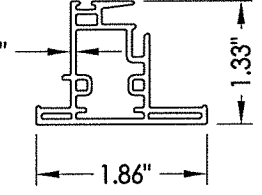
5 MEETING RAIL
