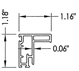
2 SASH STILE/RAIL
