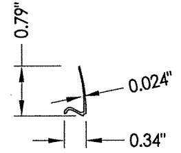
7 GLAZING BEAD
